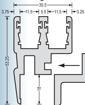
Type 1 Clamp Ring 3-10mm structure
