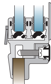
Double Sliding Type 2
