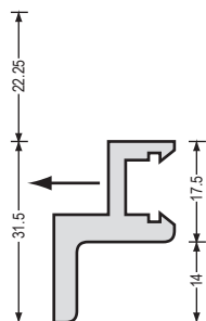
Type 2 Clamp Ring 10-20mm structure
